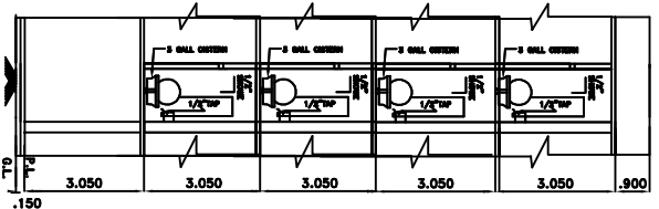
SECTION AT "C-D" SCALE - 1:100
