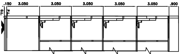
SECTION AT "A-B" SCALE - 1:100
